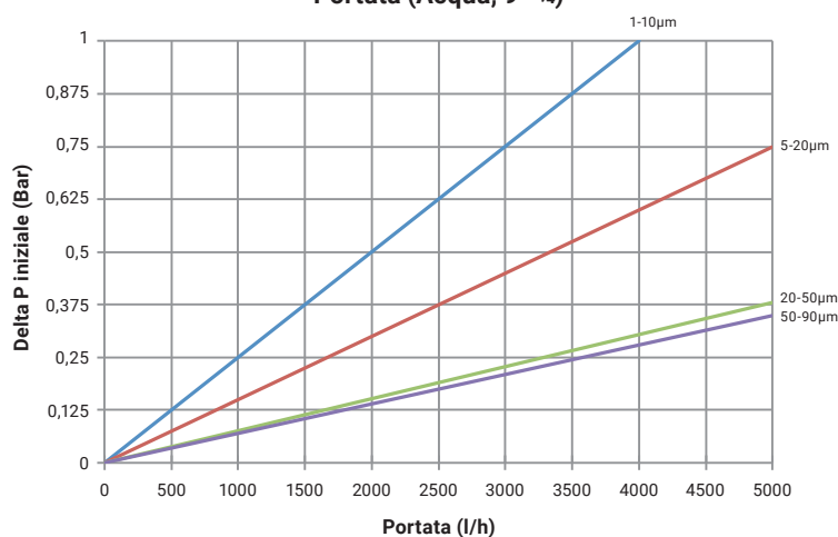
Portata (Acqua, 9" 3/4)
